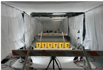
Fig. 1 Fully assembled indoor flight arena. 1
